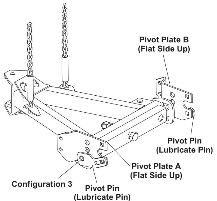
Pivot Plate Mounting and Hole Positions for Configuration 3
